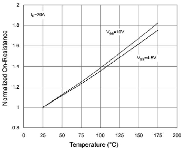
Rdson-Junction Temperature
